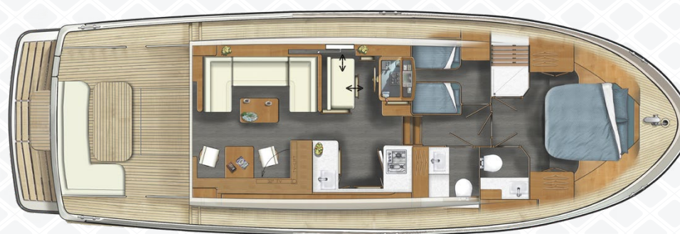
Indeling Grand Sturdy 45.0 Sedan
